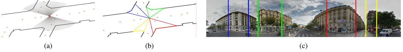
Figure 2: Overview of data generation from Google Street View images and cadastre maps. We first (a) cast 30m rays to the sides of each Street View capture location at 1^\circ intervals, then (b) compute intersections with facades and select the widest view, and (c) project onto the panoramas and crop and warp the facade images according to Street View metadata.
